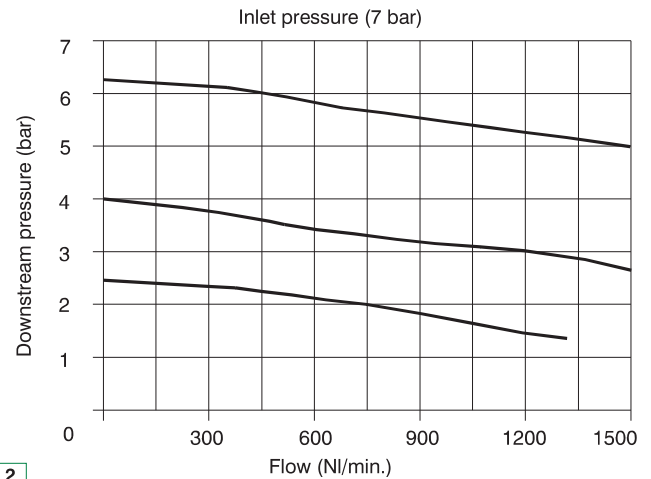
Flow rate curves
